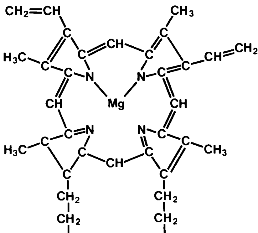
Chlorophyll Molecule
