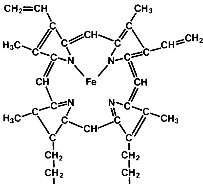
Blood Molecule
